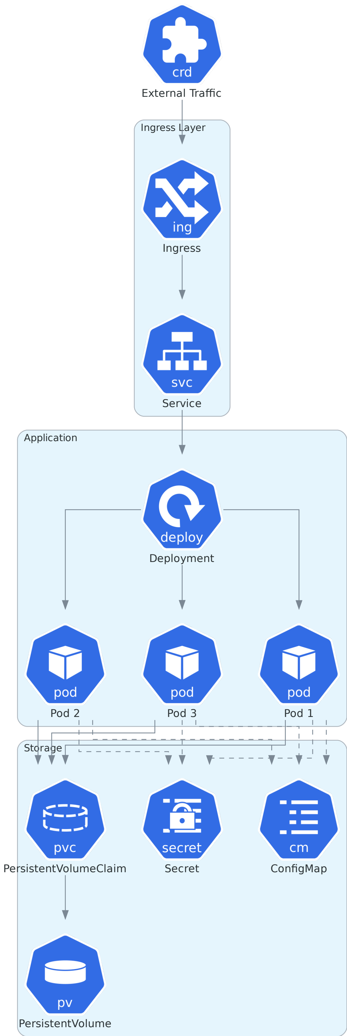
Kubernetes Deployment
